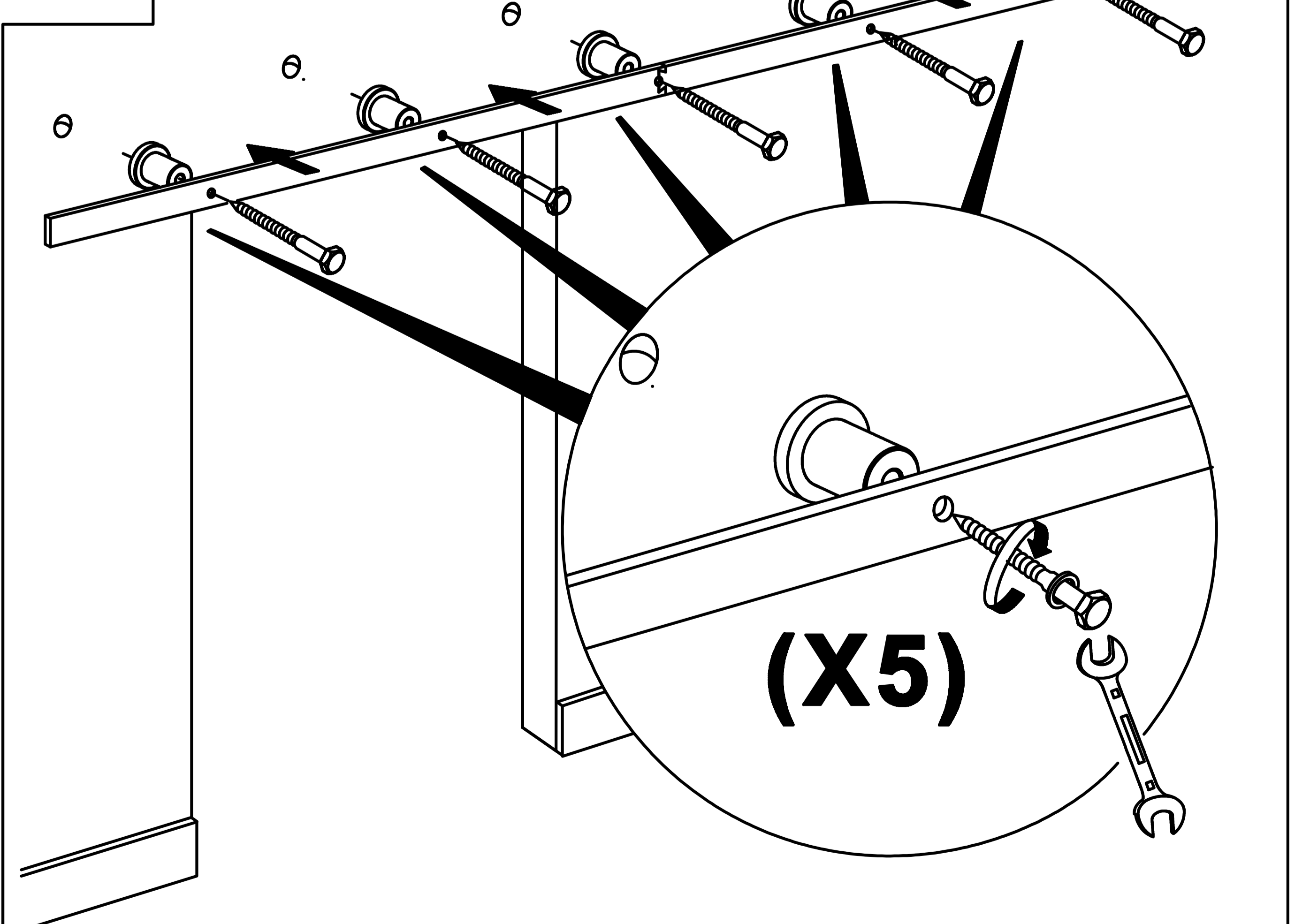
2B For drywall installation with support structure
