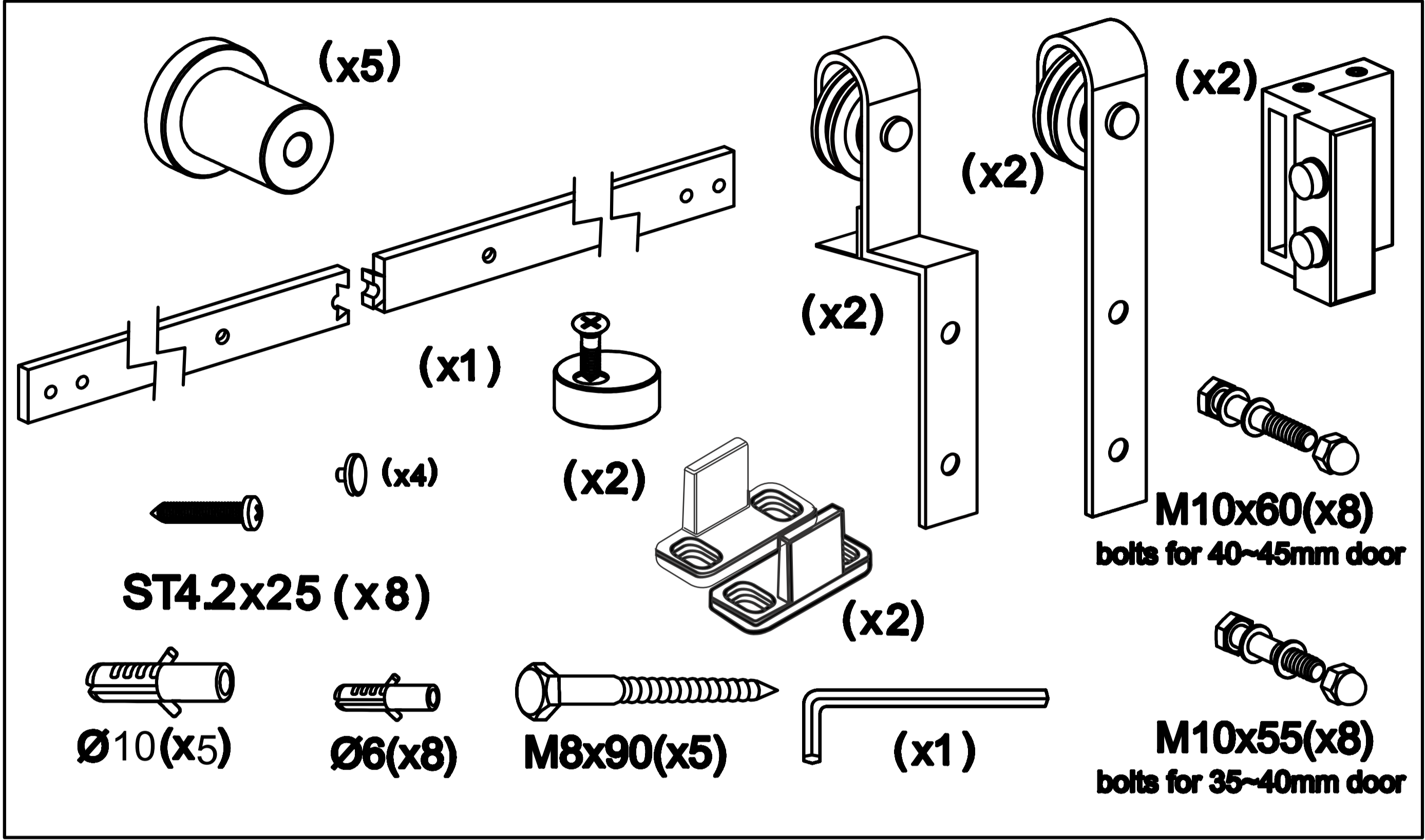
1B For drywall installation with support structure
