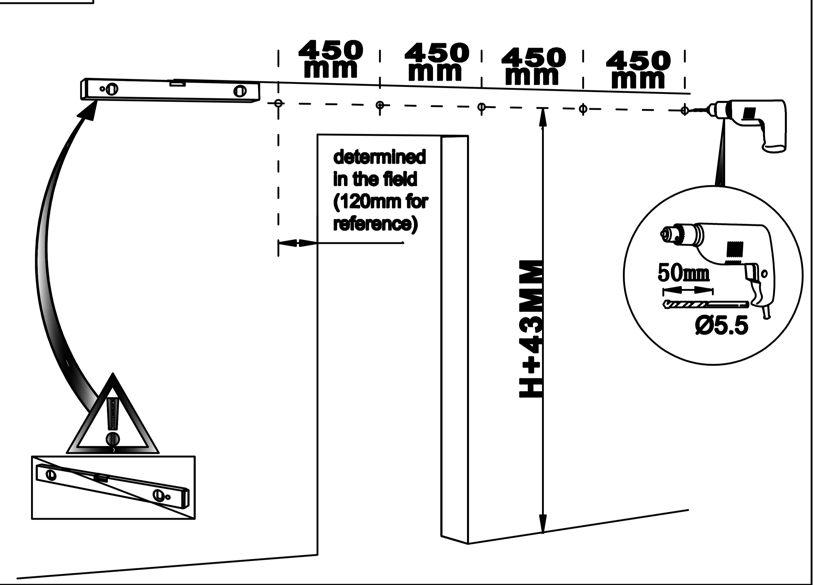
2B For drywall installation with support structure
